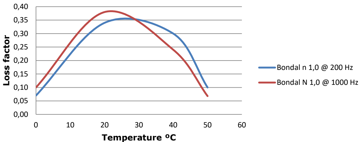
Loss factor Bondel Steel
